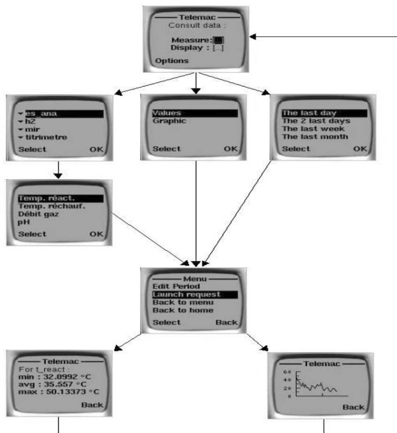
Figure 6 WAP access to the current data recorded by the plant and stored in the database
