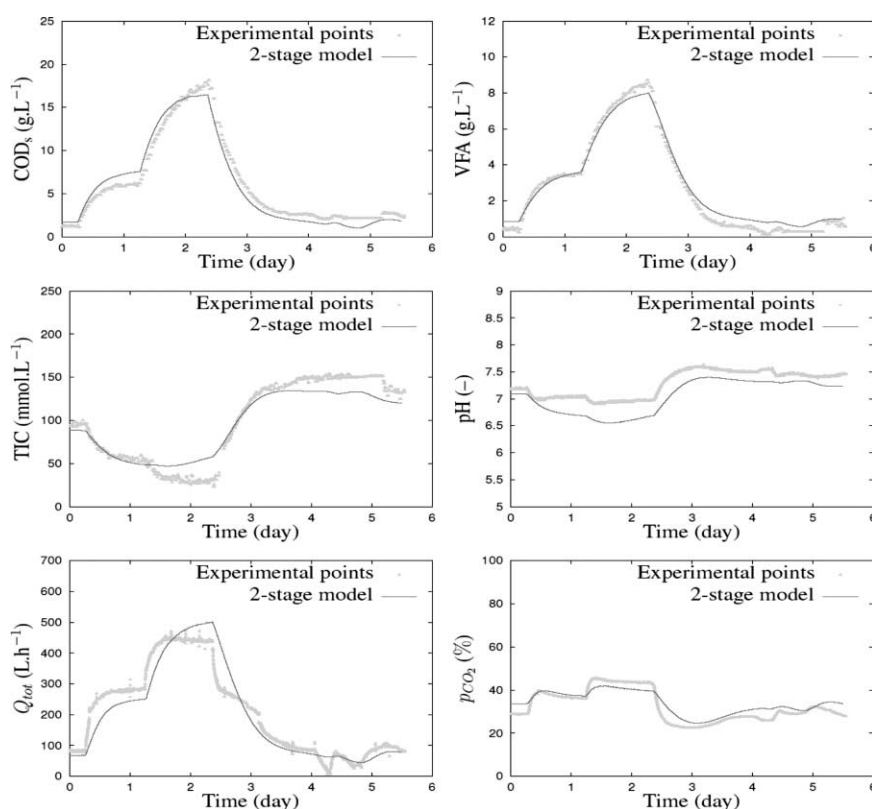
Figure 4 Experimental process overloading on a fixed bed digester processing wine vinasses. Comparison between sensor measurements and model predictions
