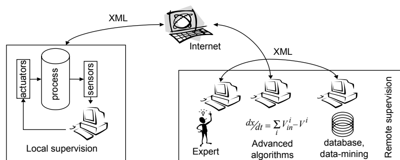
Figure 1 The overall architecture of the TELEMAT supervision system
