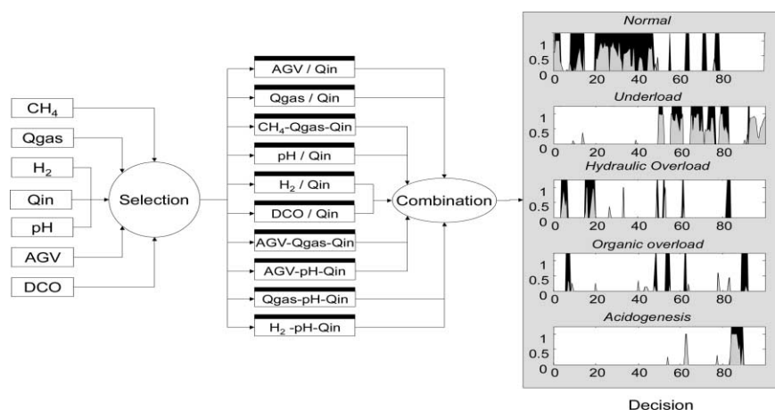
Figure 5 Illustration of the results provided by the TELEMAC fault detection and diagnosis system
